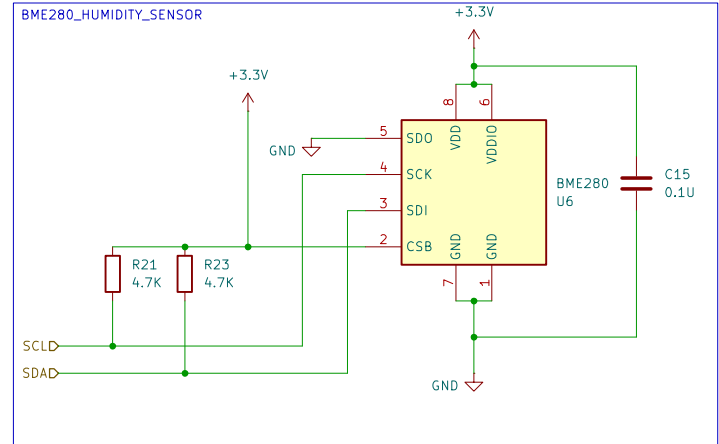
BME280_HUMIDITY_SENSOR
