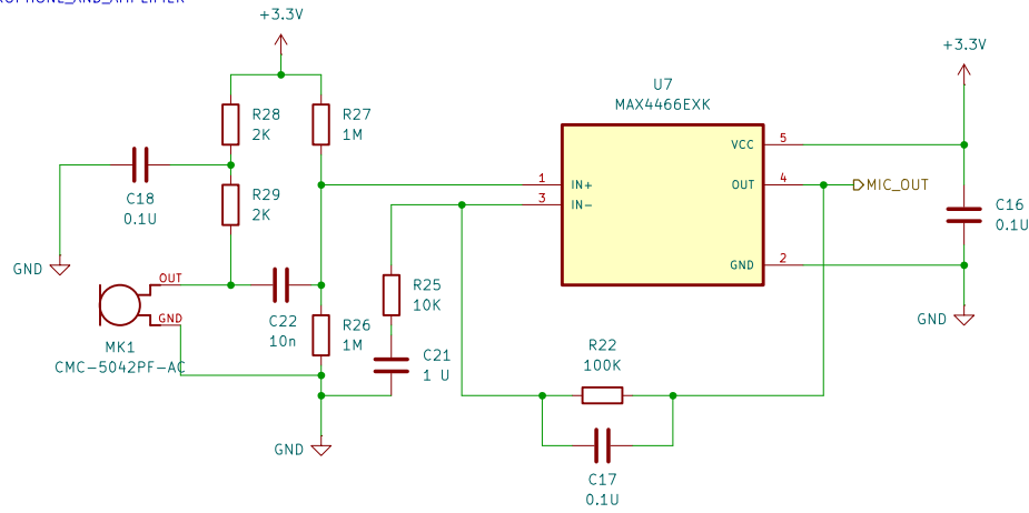
MICROPHONE_AND_AMPLIFIER
