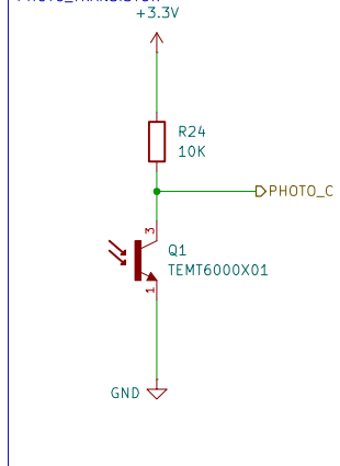
PHOTO_TRANSISTOR
